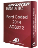
ADS222 Software
